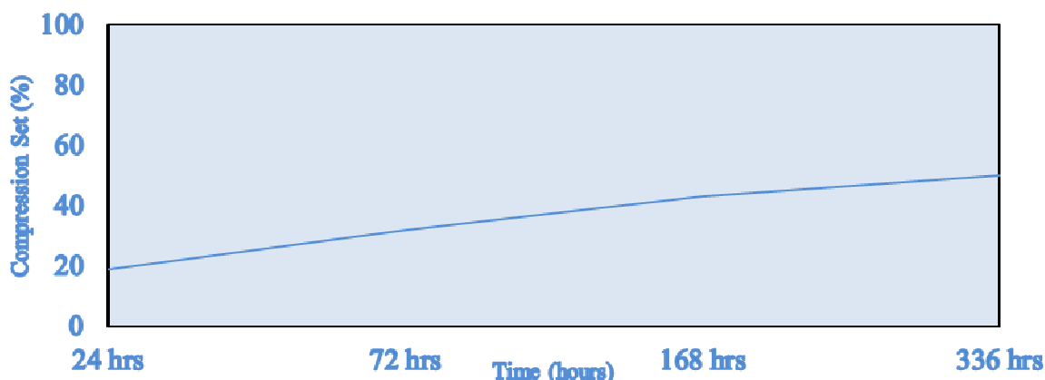
Typical Compression Set Values in Air @ 100^{\circ}\text{C} Under 25% Strain ISO 815
